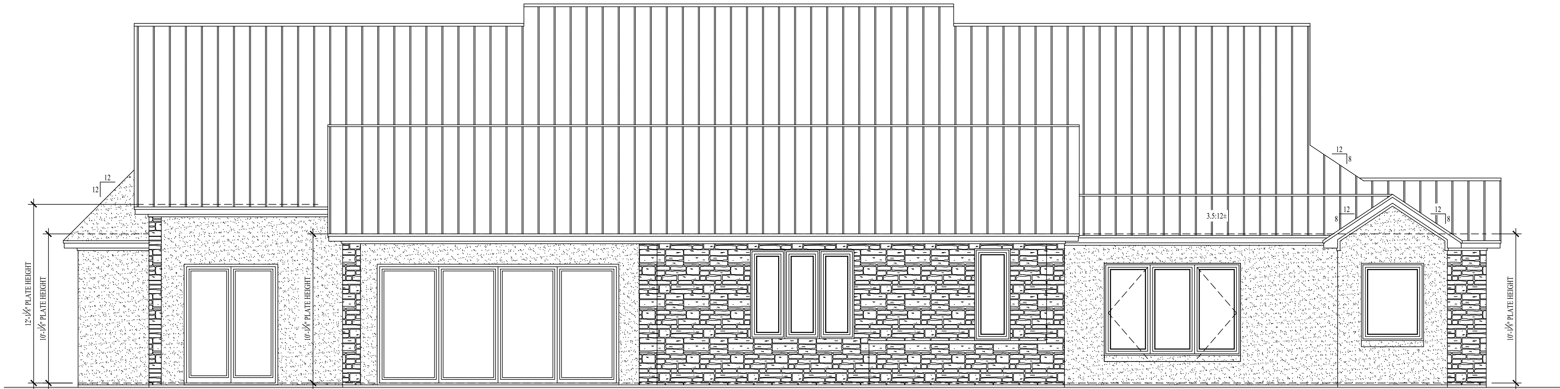
REAR ELEVATION
